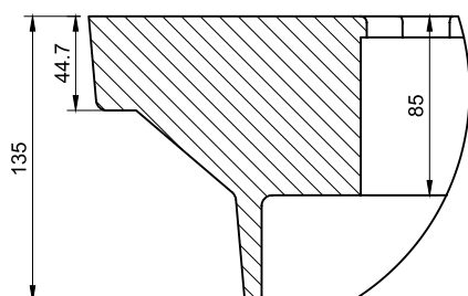
C (1:2)
