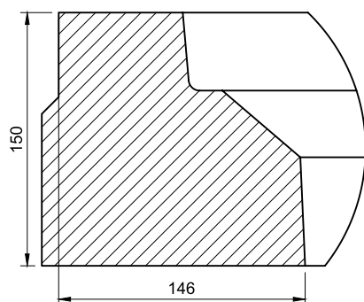
D (1:2)
